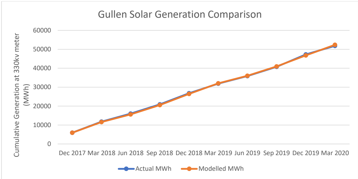
Figure 2 - Comparison of Gullen Solar Actual and Predicted Cumulative Generation
