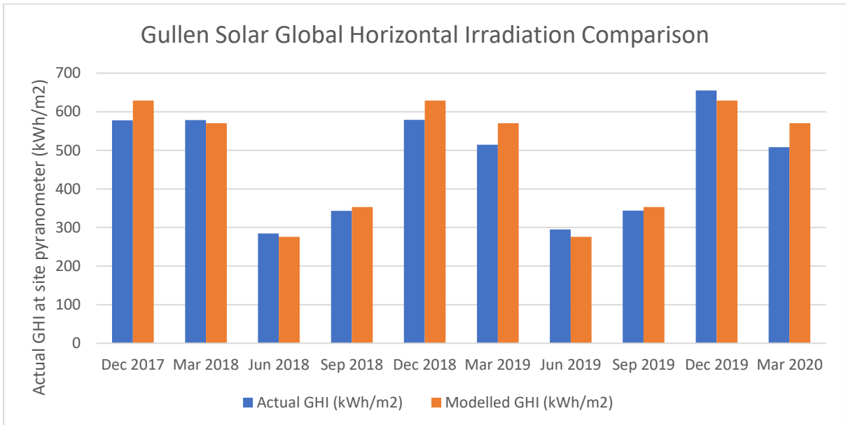
Figure 3 - Comparison of Gullen Solar Actual and Predicted GHI by Month
