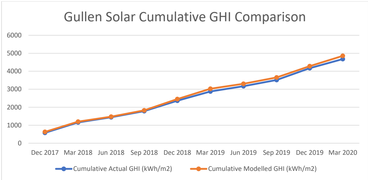
Figure 4 - Comparison of Gullen Solar Actual and Predicted Cumulative GHI
