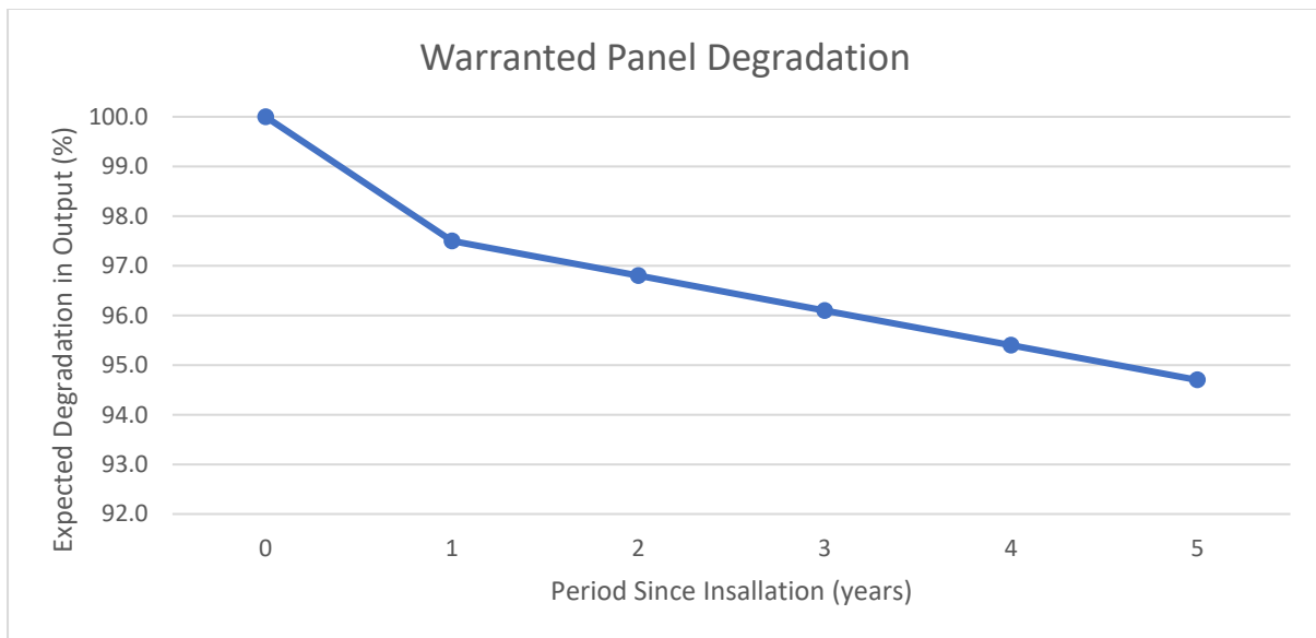
Figure 12 – Expected Panel Degradation
