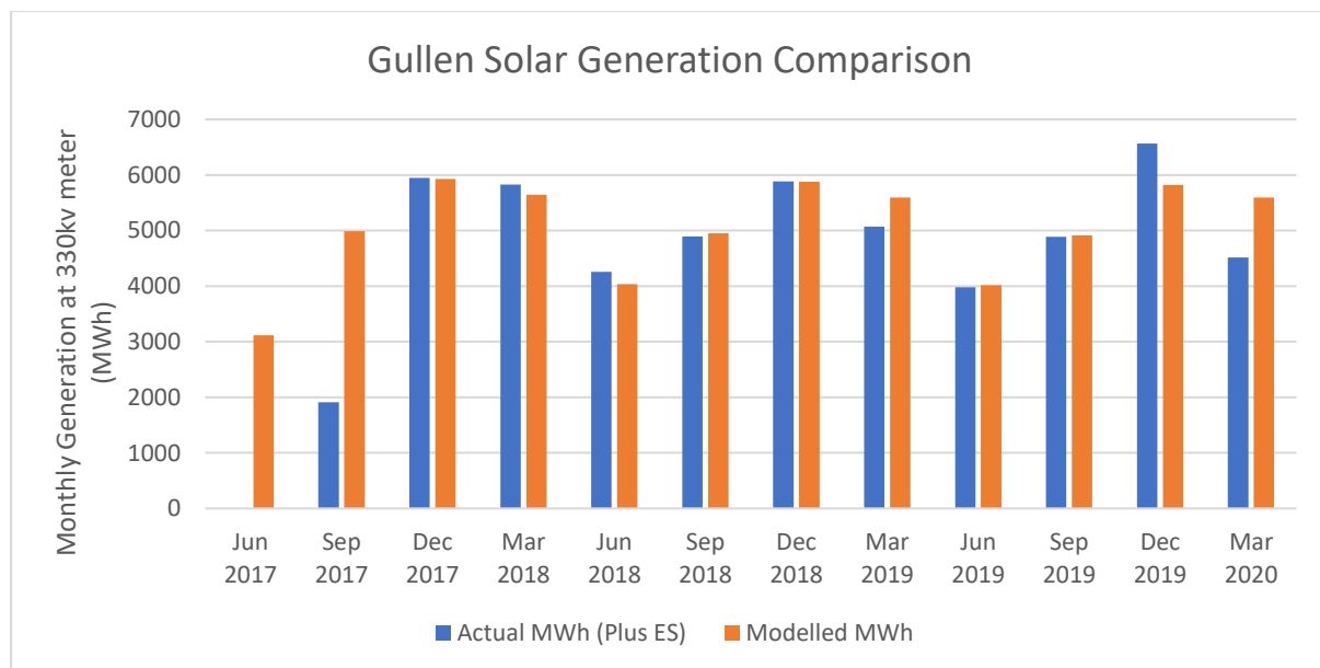
Figure 1 – Comparison of Gullen Solar Actual and Predicted Generation by Month
