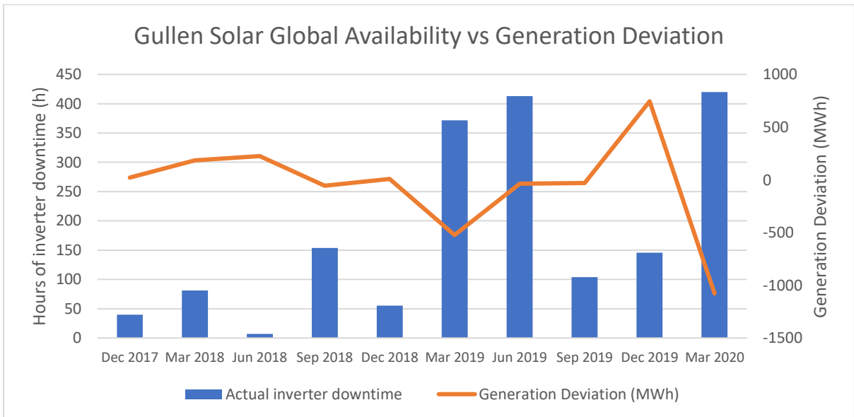
Figure 5 – Comparison of Actual and Forecast Generation Deviation to Solar Inverter Downtime
