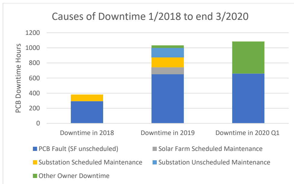
Figure 9 – Causes of Solar Farm Downtime
