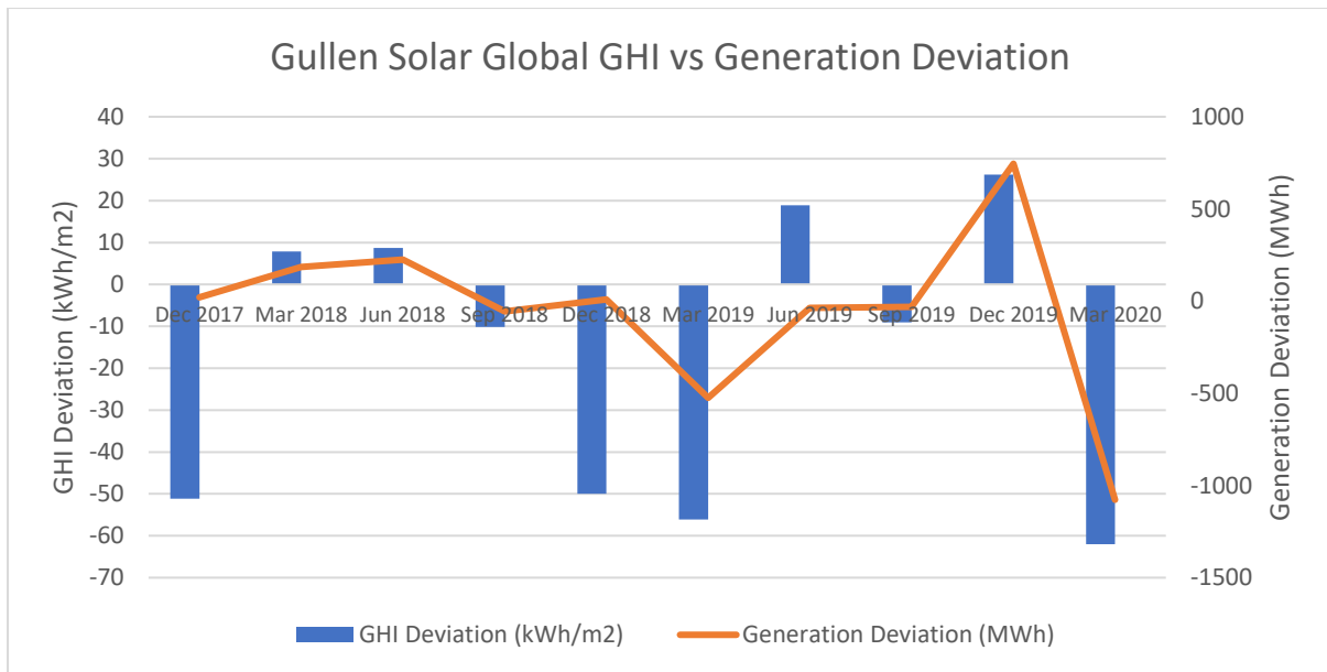
Figure 6 - Comparison of Actual and Forecast Generation and GHI Deviation
